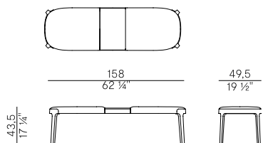
942/01 panca \ bench
