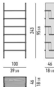
LIBRERIA CM 100X46 H243 - MOD. A BOOKCASE CM 100X46 H243 - MOD. A
